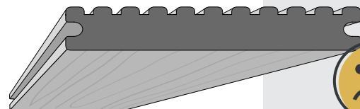
SOLID & UNCAPPED BOARD WITH GROOVE FOR HIDDEN FIXINGS
