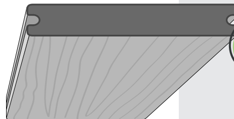
SOLID & CAPPED BOARD WITH GROOVE FOR HIDDEN FIXINGS
