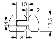
DETAIL B SCALE 2 : 3
